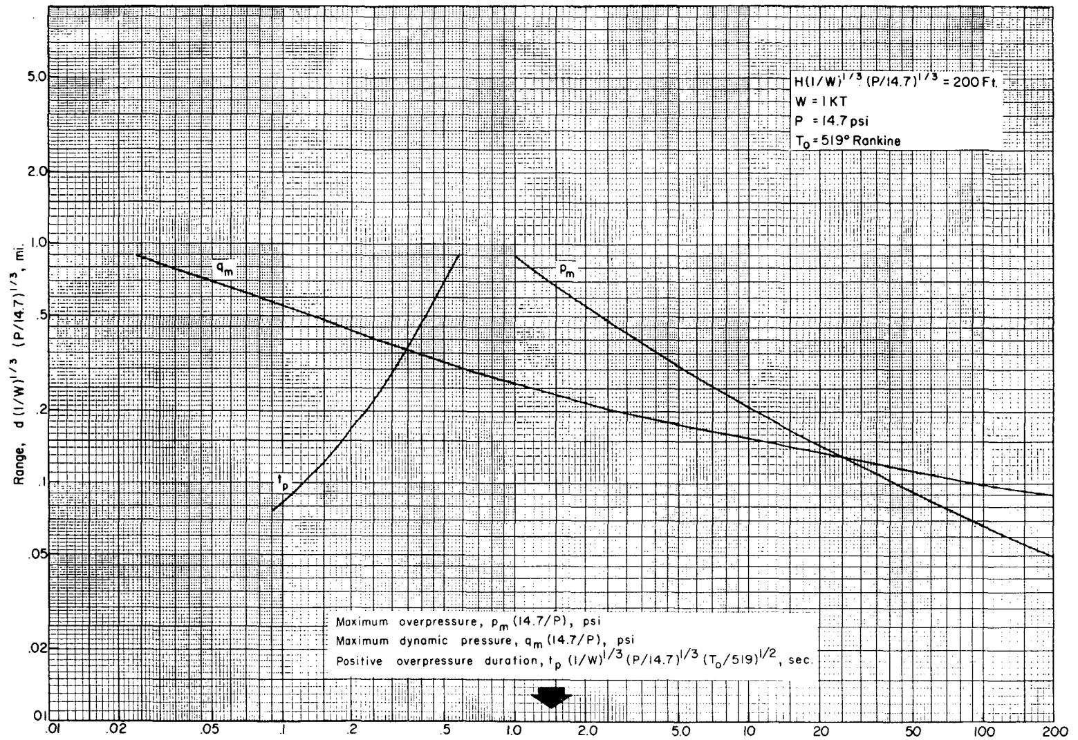
Fig. 2.3—Scaled blast parameters for a scaled height of burst of 200 ft as a function of scaled range. These are plots of Eqs. 2.24, 2.26, and 2.28 given in Table 2.3.
